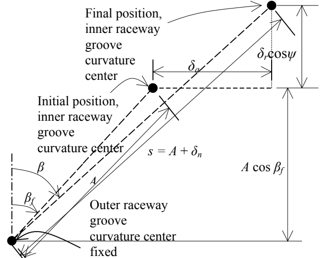
Fig. 7 Initial and final curvature centers positions at angular position \psi , with and without applied load
